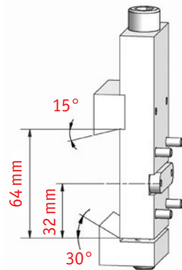
Standard dovetail adapter (clamping from below)
