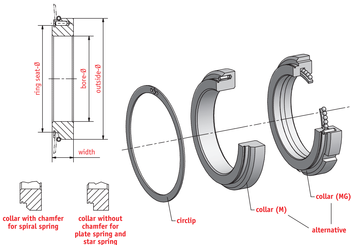
Index for collar (M)
