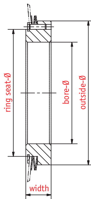
Representation: collar with plate spring
