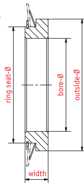
Representation: collar with star spring
