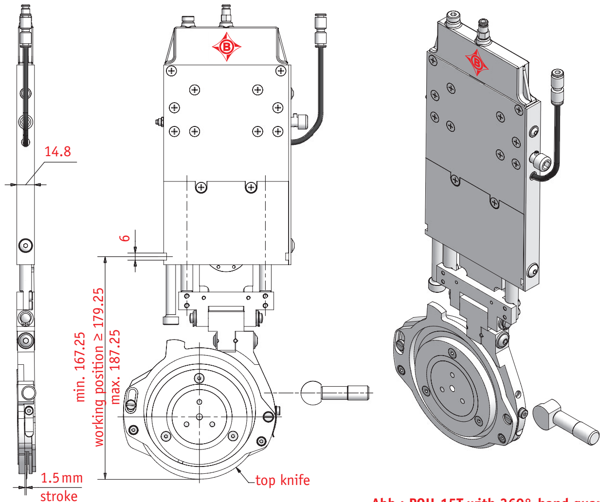
Abb.: POH-15T with 360°-hand guard
